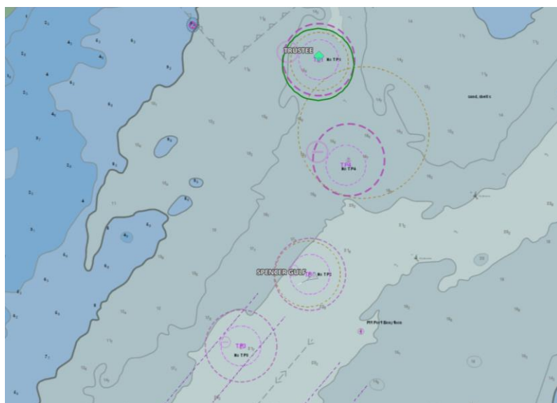
Figure 2 Chartlet of Offshore Transshipping Locations
